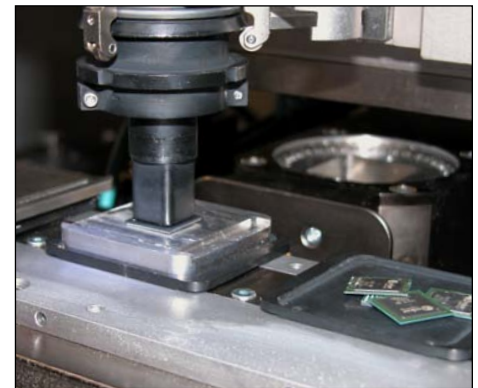
SOLDER PASTE DIP & DROP OFF TRAY
